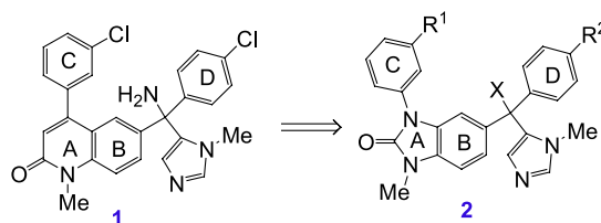
Figure 1. Modifications of tipifarnib ( 1 ) lead to novel inhibitors ( 2 ) of FTase.
