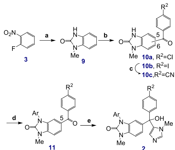
Scheme 2. Reagents and conditions: (a) (i) MeNH 2 , MeOH/H 2 O, reflux, overnight, 98%; (ii) H 2 , 10% Pd–C, MeOH, rt, 30 min, 98%; (iii) CDI, CH 2 Cl 2 , reflux, 3 h, 73%; (b) 4-halobenzoyl chloride (excess), AlCl 3 , neat, 150 °C, overnight, 46–73%, 1:1 mixture of 5- and 6-isomers; (c) Zn(CN) 2 , Pd(P(Ph) 3 ) 4 , DMF, 80 °C, 3 h, 98%; (d) ArB(OH) 2 , Cu(OAc) 2 , Et 3 N, CH 2 Cl 2 , rt, 3 days, 12–43%; (e) 1-methyl-2-TES-imidazole, tert -BuLi, THF, –78 °C, 0.5 h, then 11 , –78 °C to rt, 4 h; (ii) MeOH, 10% HCl, rt, 0.5 h, 19–87%.
