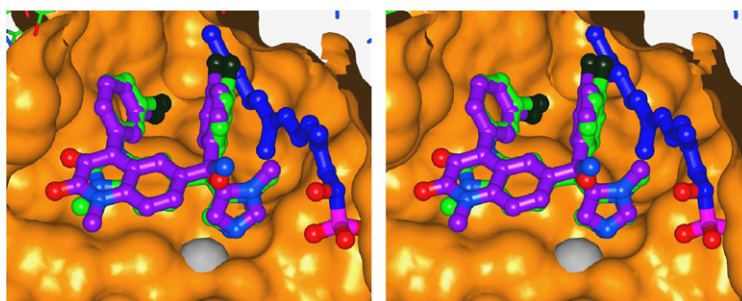
Figure 2. Stereo view of an overlay of a model of compound 2a (in green) over the X-ray crystal structure of tipifarnib ( 1 ) 5 (in purple) in complex with FTase in the active site. Zn 2+ is shown in gray and hydroxy farnesylpyrophosphate in blue.
