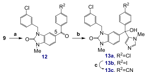
Scheme 3. Reagents and conditions: (a) (i) 3-chlorobenzyl chloride, NaH, DMF, rt, 1 h, 95%; (ii) 4-halobenzoyl chloride (excess), AlCl 3 , neat, 100 °C, overnight, 31–34%; (b) 1-methyl-2-TES-imidazole, tert -BuLi, THF, –78 °C, 0.5 h, then 12 , –78 °C to rt, 4 h; (ii) MeOH, 10% HCl, rt, 0.5 h, 85–94%; (c) Zn(CN) 2 , Pd(P(Ph) 3 ) 4 , DMF, 80 °C, 3 h, 62%.
