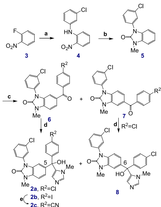
Scheme 1. Reagents and conditions: (a) 3-chloroaniline, KF, 180 °C, 44 h, 97%; (b) (i) SnCl 2 ·2H 2 O, HCl, EtOH, 0 °C–rt, overnight, 97%; (ii) CDI, CH 2 Cl 2 , reflux, 2 h, then EtOH, reflux, 2 h, 73%; (iii) MeI, NaH, DMF, rt, 1 h, 94%; (c) 4-halobenzoyl chloride (excess), AlCl 3 , neat, 150 °C, overnight, 17–40% ( 6 ), 21% ( 7 , X = Cl); (d) (i) 1-methyl-2-TES-imidazole, tert -BuLi, THF, –78 °C, 0.5 h, then 6 or 7 , –78 °C to rt, 4 h; (ii) MeOH, 10% HCl, rt, 0.5 h, 62–87% ( 2 ), 42% ( 8 ); (e) Zn(CN) 2 , Pd(P(Ph) 3 ) 4 , DMF, 80 °C, 3 h, 71%.
